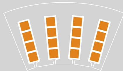
High Slot-Fill Square Wire
